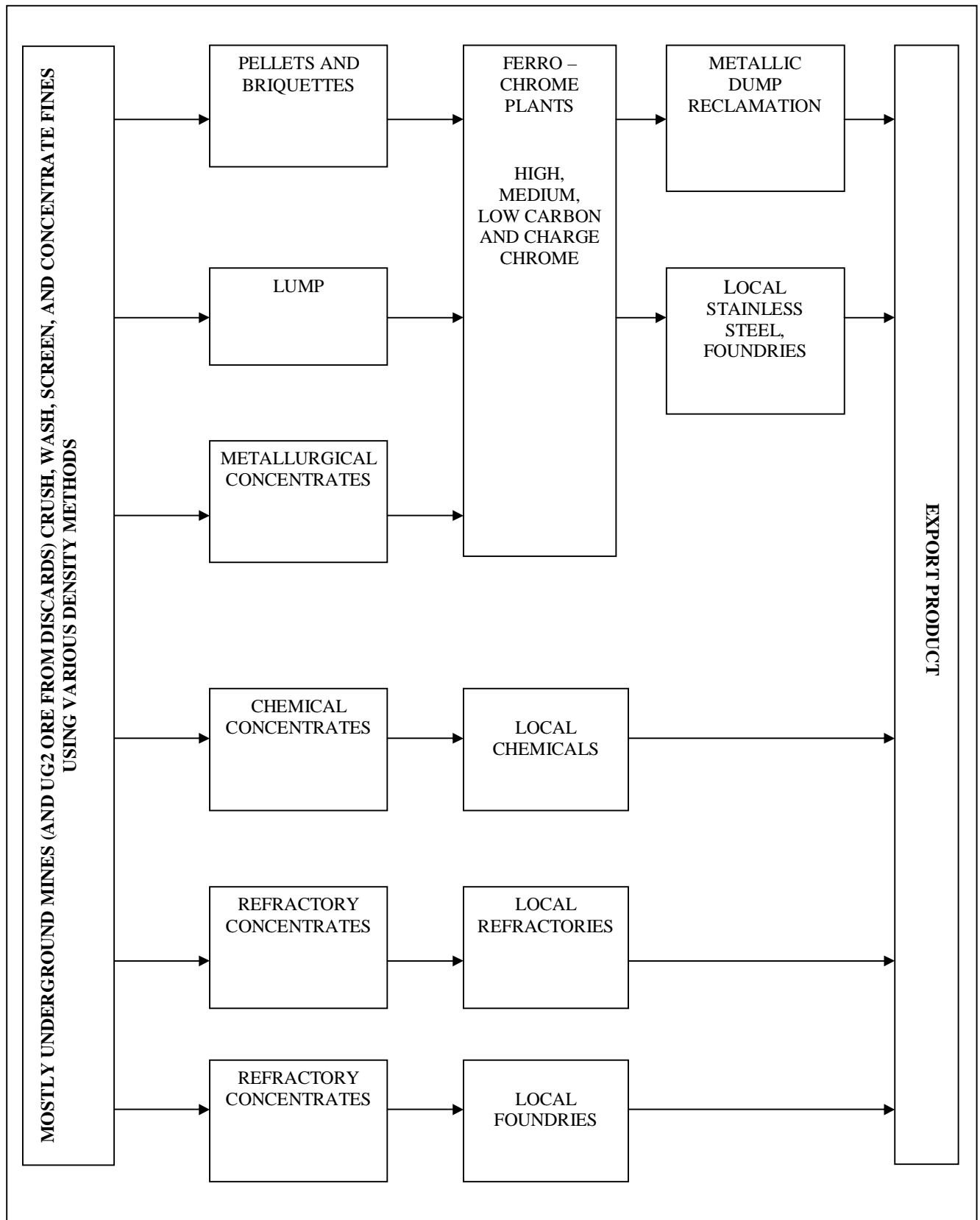
FIGURE 1: CHROME FLOW DIAGRAM
